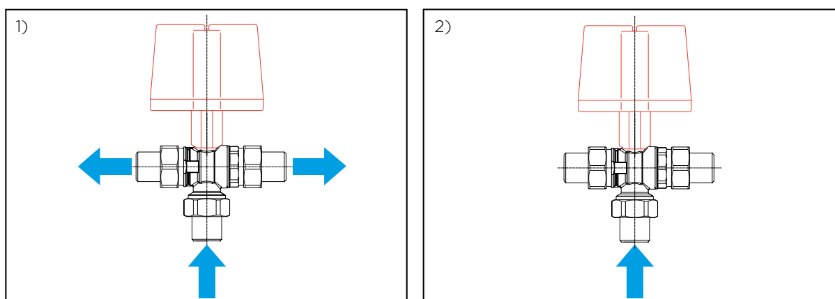
1) Schema a tre vie a "T" in posizione ON. Three-way T-port diagram in ON position.
